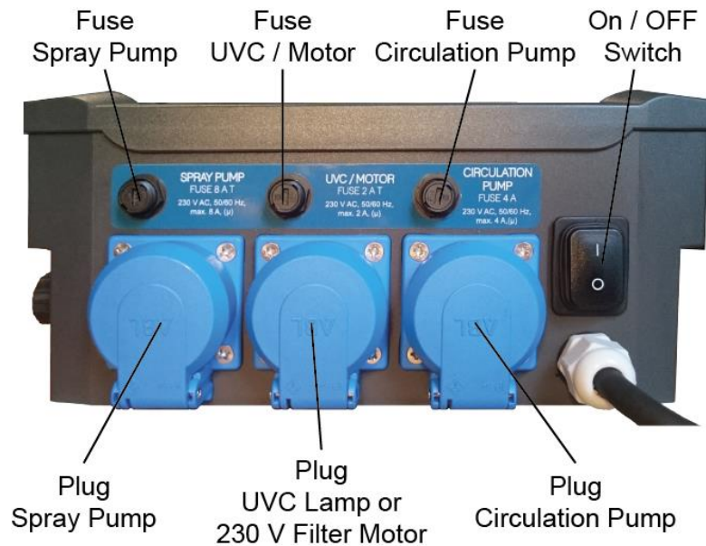
Fig. 3: View at the lower side of the FILTER|CONTROL.
