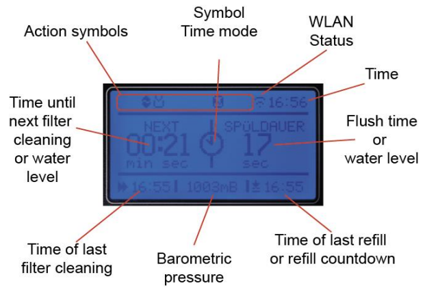
Fig. 5: The display of the FILTER|CONTROL.
