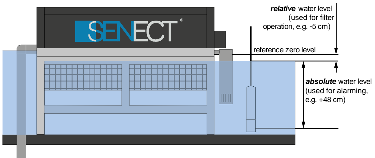
Fig. 2: Relative water level vs. absolute water level.
