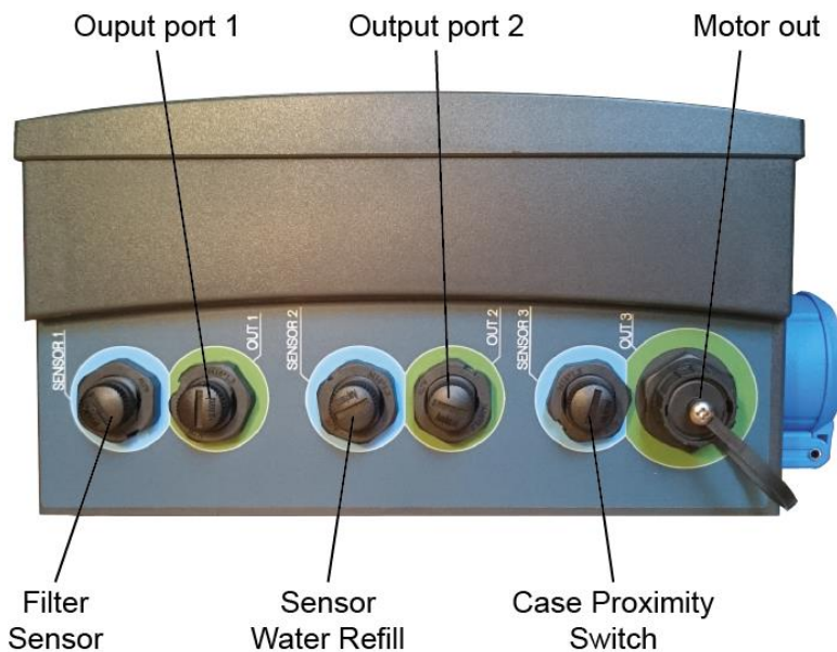
Fig. 2: Sensor and actuator ports of the FILTER|CONTROL.
