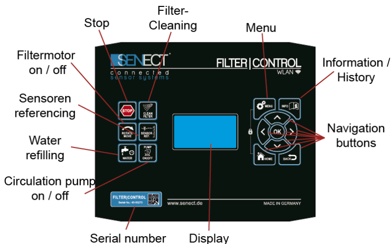
Fig. 6: Buttons of the FILTER|CONTROL.
