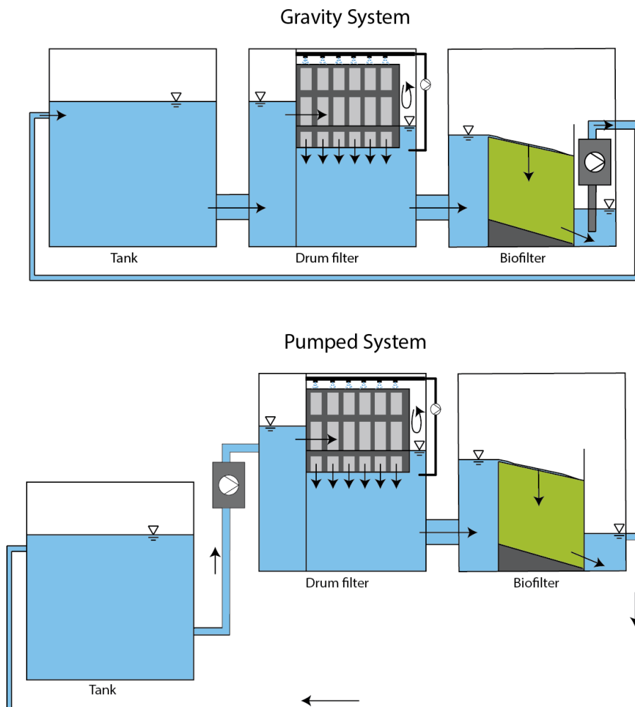
Fig. 4: Sketch showing the general two hydraulic systems in which drum filter are operated.
